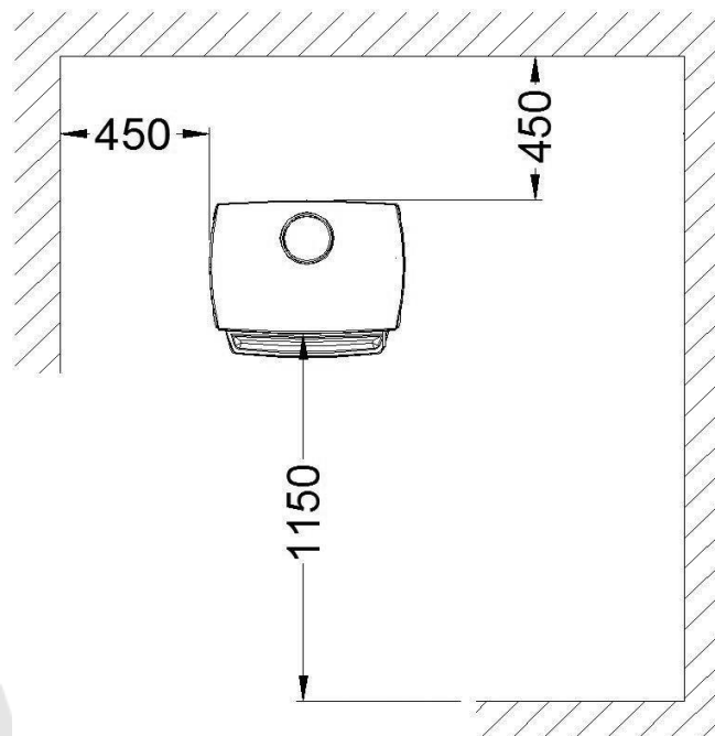
FIG. 6 - SAFETY DISTANCES
