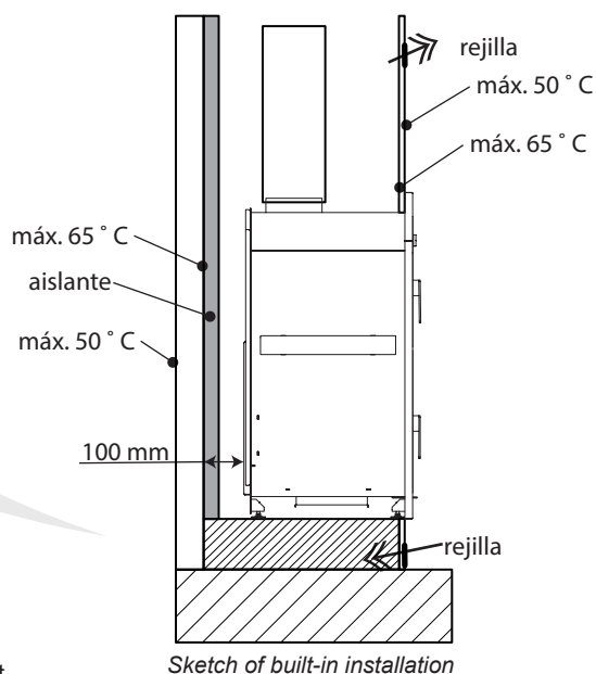
Sketch of built-in installation
