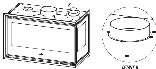
Installation of outlet channels
