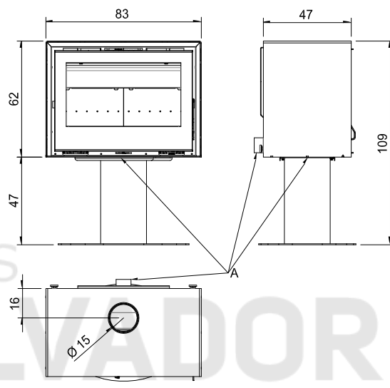
RI 80 con Pie/ RI 80 with Stand.
